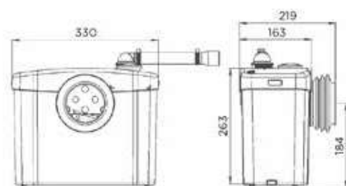
Dimensions (mm)
